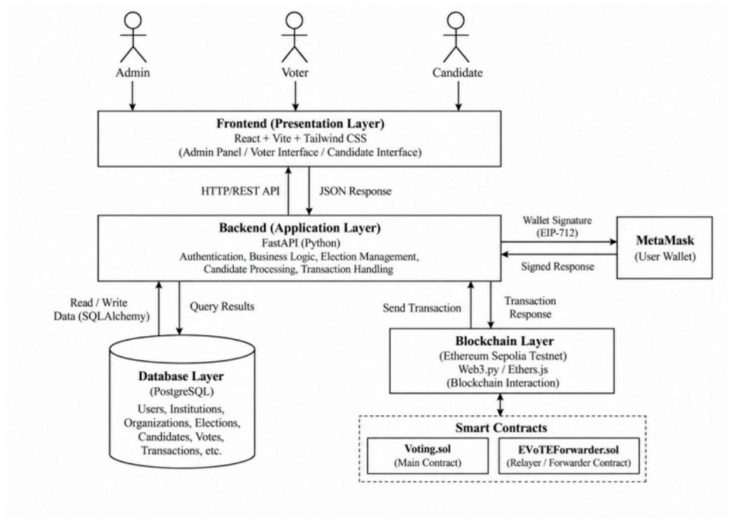
Fig 2: System Architecture of the Blockchain Based Voting System
