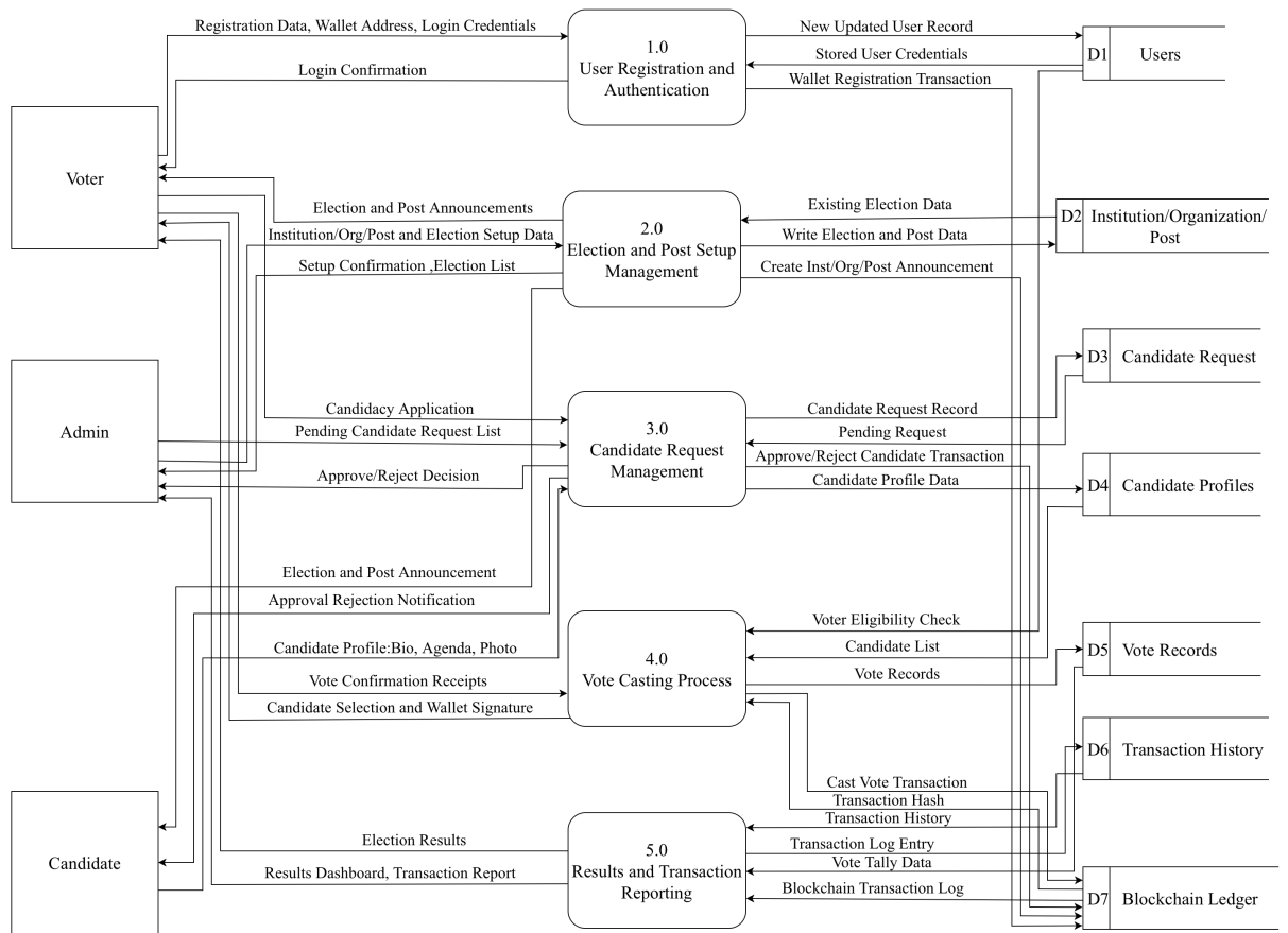
Fig 4: DFD Level 1 of the Blockchain Based Voting System
