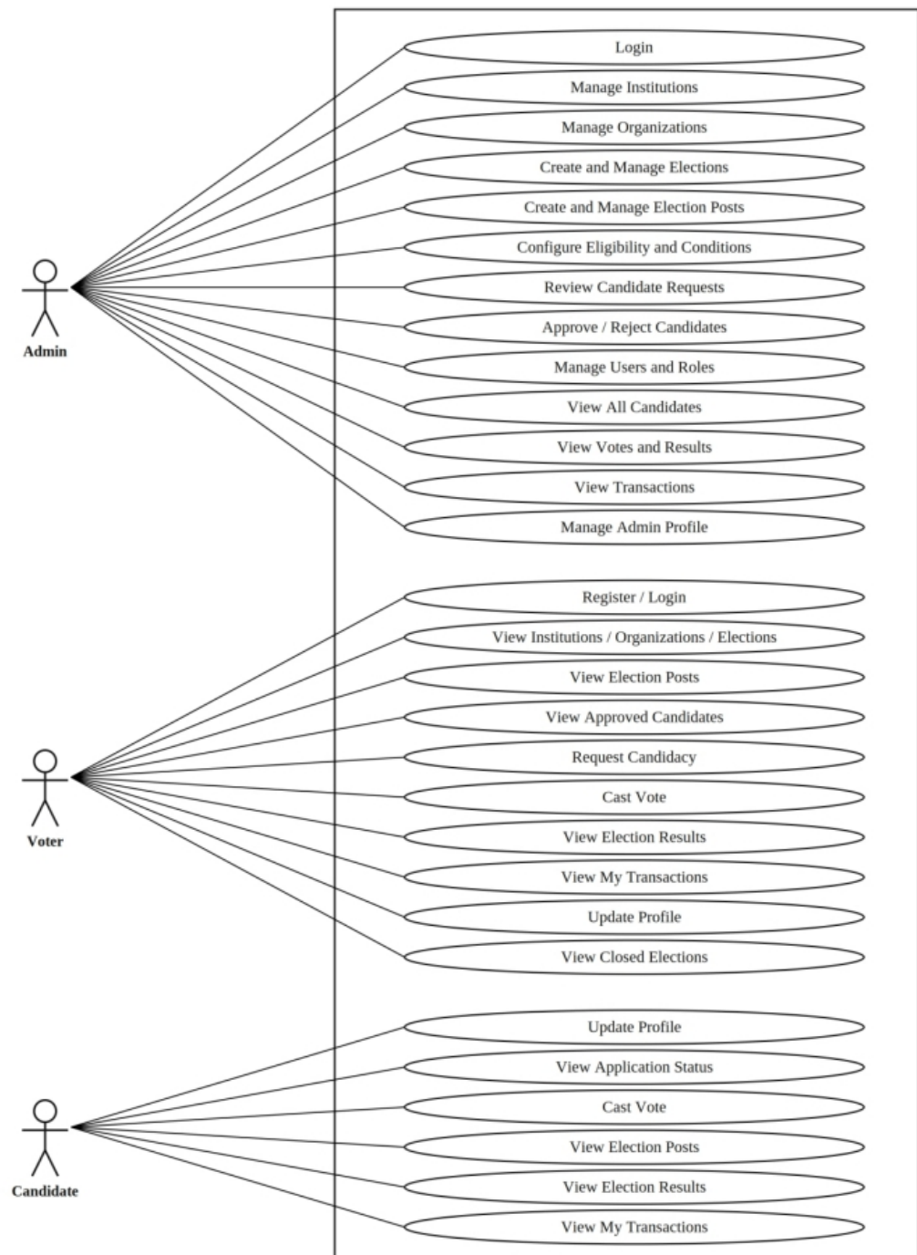
Fig 1: Use-Case Diagram of the Blockchain Based Voting System
