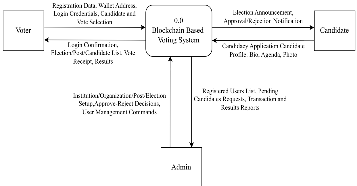
Fig 3: DFD Level 0 of the Blockchain Based Voting System
